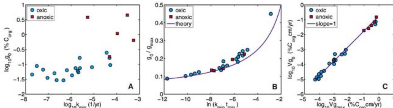
Fig. 3. (A) The 23 k_{\min} , g_0 pairs used to rescale the data of Fig. 2B. The cores underlying anoxic waters (red squares) are associated with higher k_{\min} and g_0 . (B) The same k_{\min} , g_0 pairs plotted with dimensionless rescaled axes g_0/g_{\max} and \ln(k_{\min} t_{\min}) . The vertical axis is proportional to burial efficiency. The smooth curve is the theoretical prediction of Eq. 4, which contains no free parameters. (C) Log-log plot of the sediment fluxes Vg_0 versus Vg_{\max}
